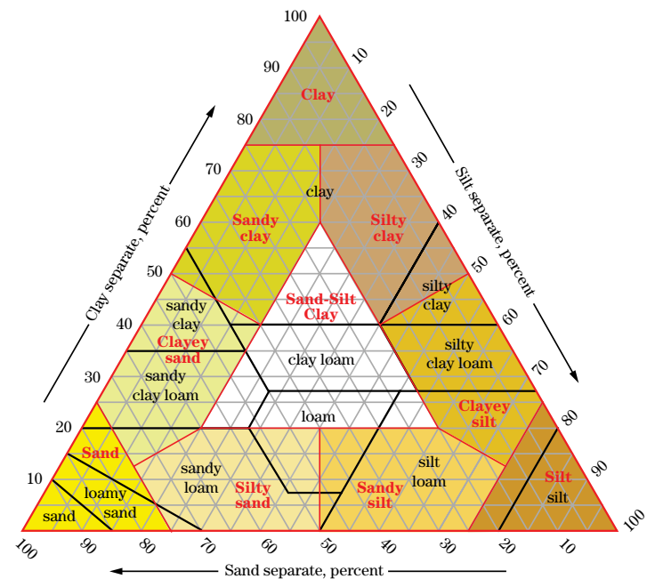
Figure 3-1 USDA textural soil classification (USDA 1951)
