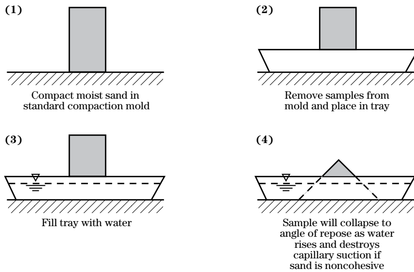
Figure 45B-2 Vaughan and Soares test for self-healing characteristics
