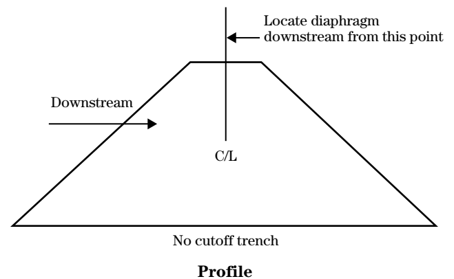
Figure 45A-14 Downstream of the centerline of the dam when no cutoff trench is used
