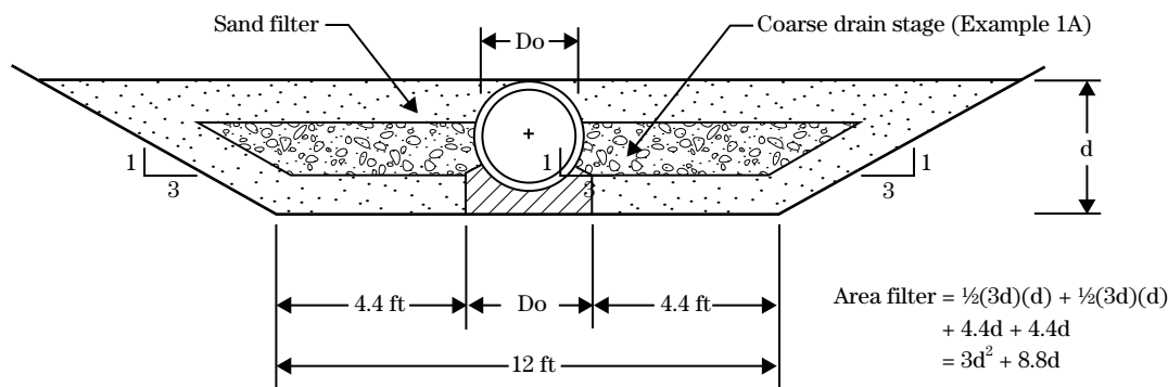
Figure 45C-4 Two-stage drain
