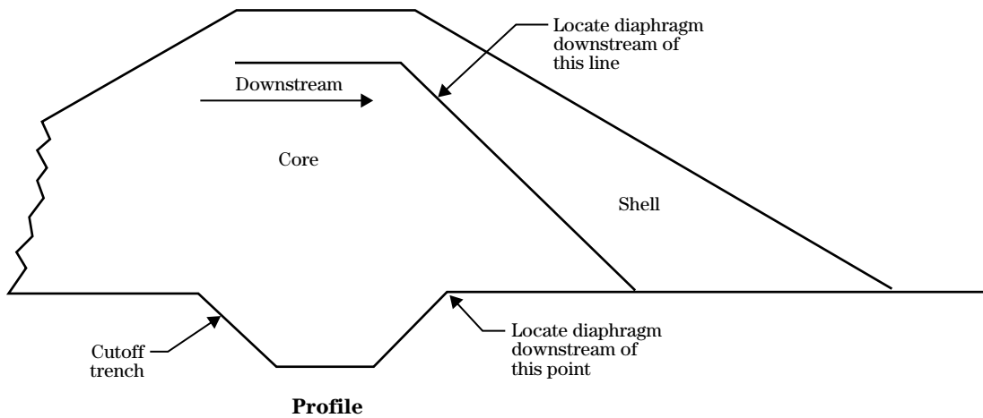
Figure 45A-16 Zoned embankments
