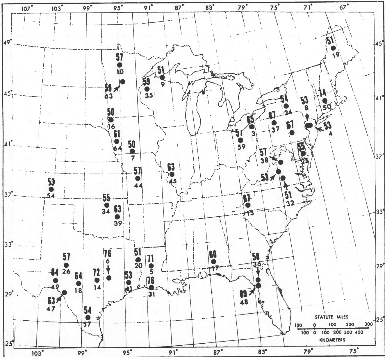
Plate 3: Observed rainfalls \geq 50% of all-season PMP, U.S. east of the 105th meridian for 1000 mi 2 48 hours. (Large number is % of PMP, small number is storm index, see table 1.)
